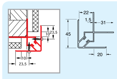
ECACE/I External / Internal Corner Profile
