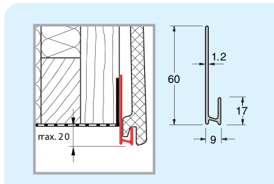
ECHSP Starting Profile P / Horizontal Starter Profile
