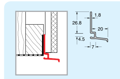
ECVSP Layering Profile / Vertical Starter Profile
