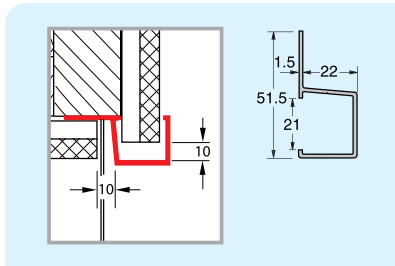
ECFP Connection Profile F
