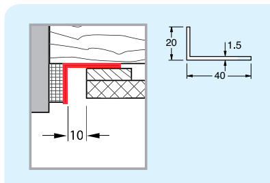
ECA40 Angle 40 x 20 * Cover angle available in 40 x 20 & 20 x 20
