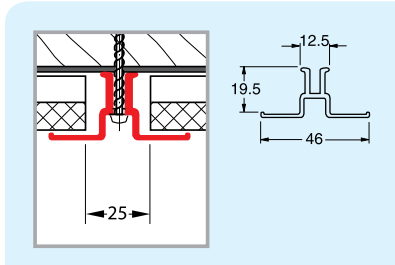
ECJCP Joint Cover Profile
